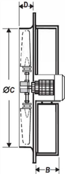
VISTA LATERAL (SIDE VIEW)
